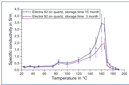
Fig. 2: Conductivity properties of Electra 92 batches stored for different times
