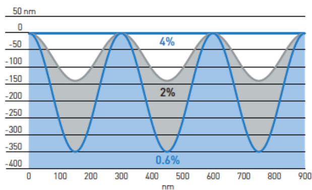
Reflectivity vs. structure depth
